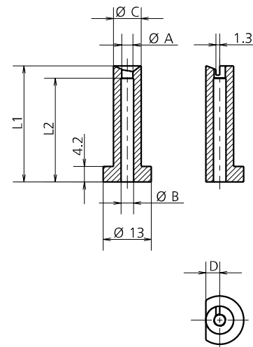
002 (8053) MATRICE / MATRIX / MATRIX HSS-62HRC
